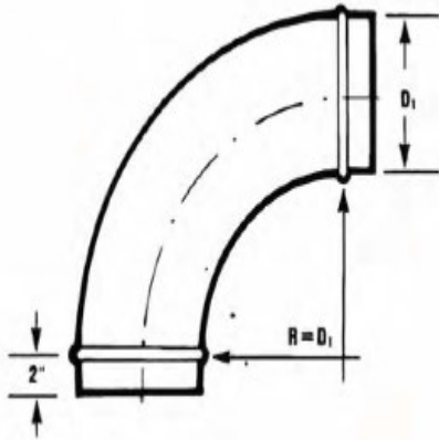
DC - 90 90° DIE STAMPED ELBOW R = 1.5 X D SPIRAL FITTINGS, INC
