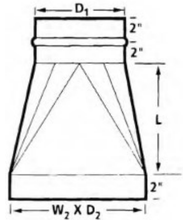
SQ 2RD SQUARE TO ROUND
