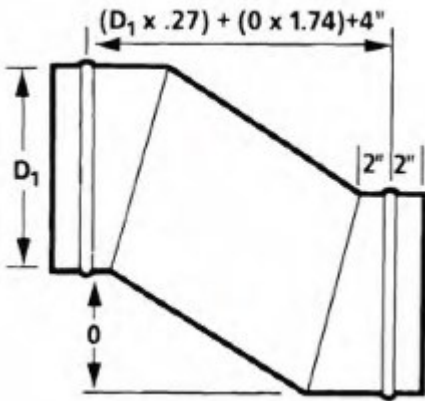
OFF OFFSET
