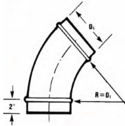
DC - 45 45° DIE STAMPED ELBOW R = 1.5 X D SPIRAL FITTINGS, INC
