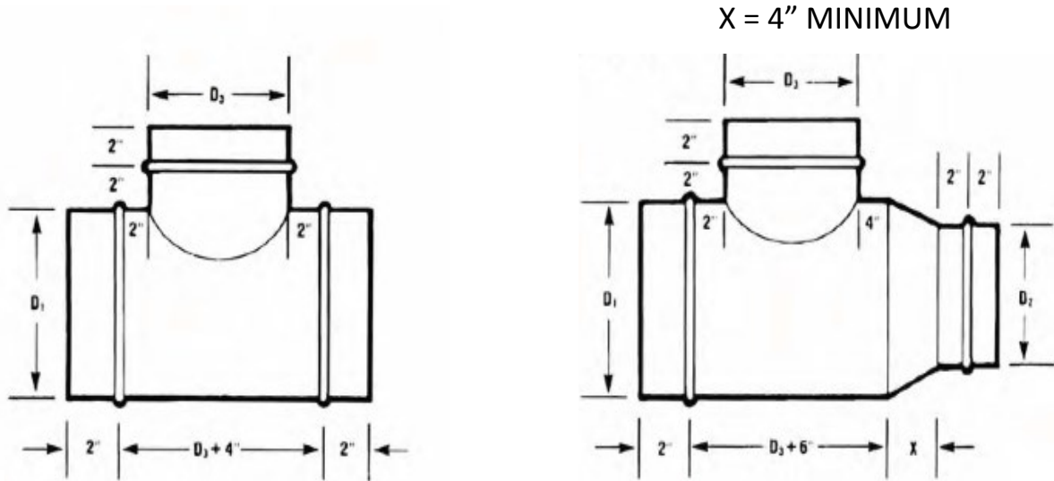
DCT - 90 90° TEE
